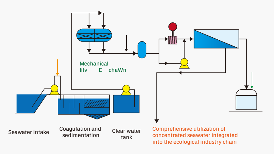
Seawater Desalination Flow Chart
